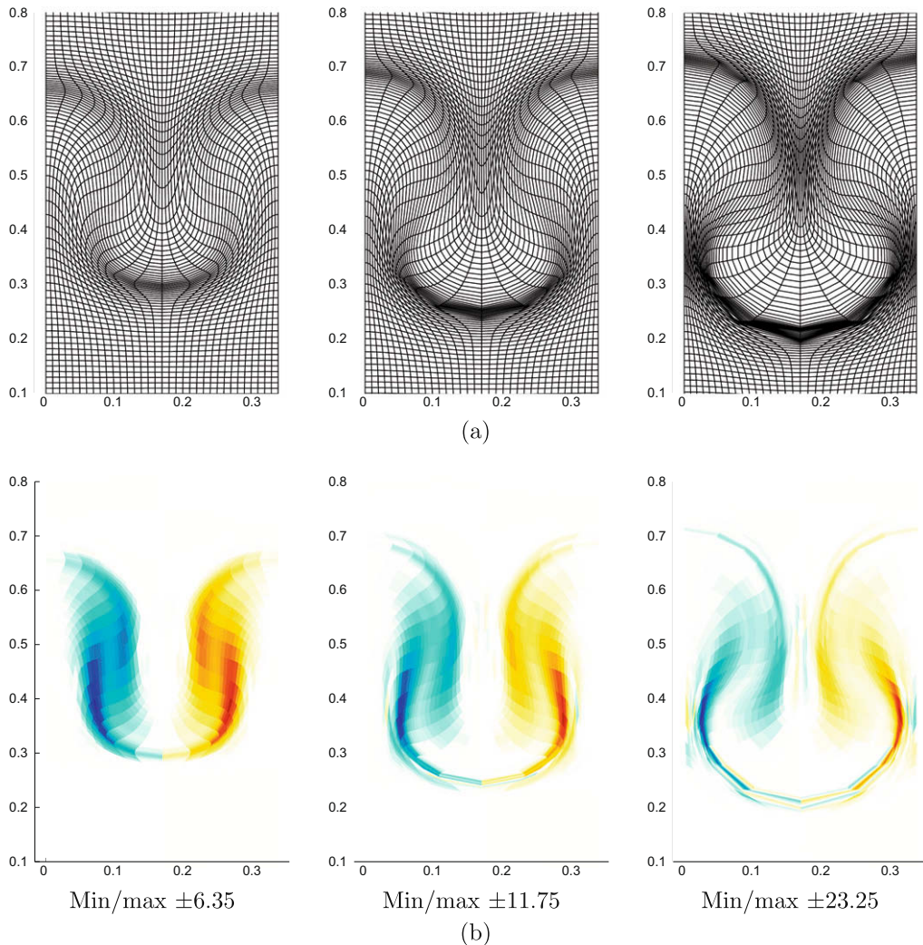
Fig. 1. Rayleigh–Taylor problem at time moments t = 7, 8, 9 – (a) Mesh fragments. (b) Vorticity color map. Color scale is from blue (minimal negative vorticity) to red (maximal positive vorticity). White color corresponds to zero vorticity. (For interpretation of the references to colour in this figure legend, the reader is referred to the web version of this article.)
